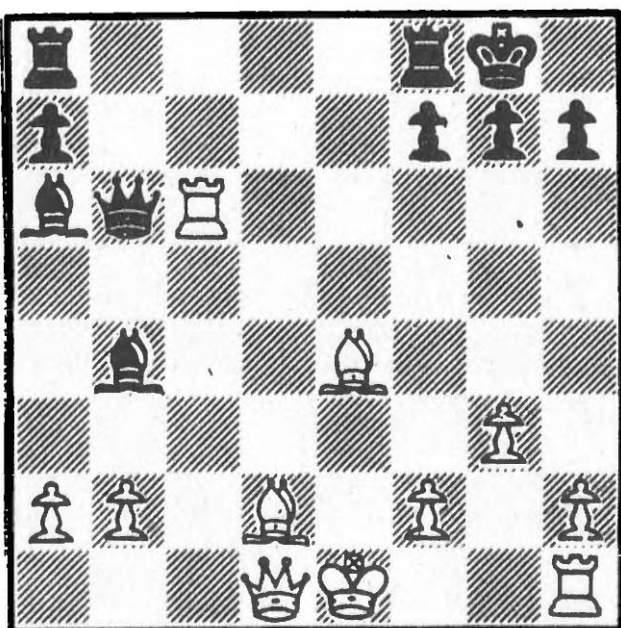
277 After 15 Rxc6
